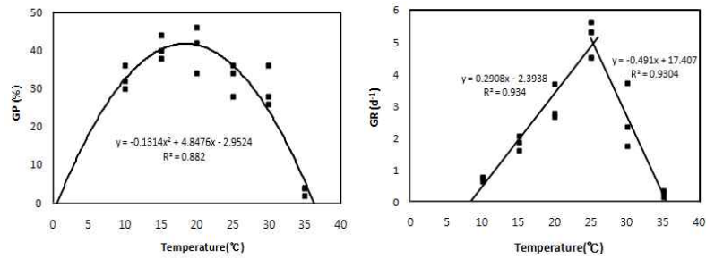
Fig. 2. Regression equations and r^2 by quadratic regression model, and linear sub- and supra-optimal models for germination percentage (GP) and rate (GR) in H. rhannodes seed as a function of temperature response, respectively.
